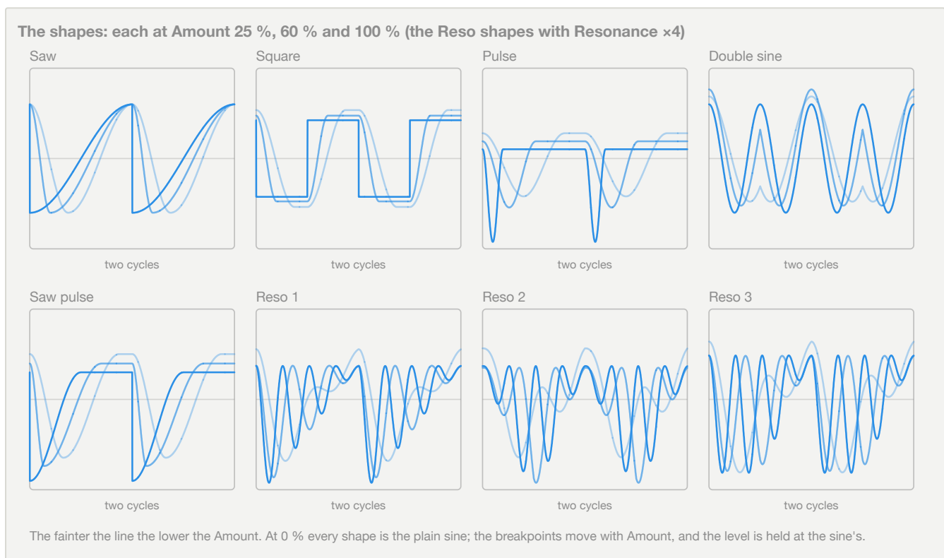
The eight shapes at three Amounts
