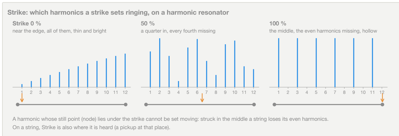
Strike: which harmonics a strike sets ringing
