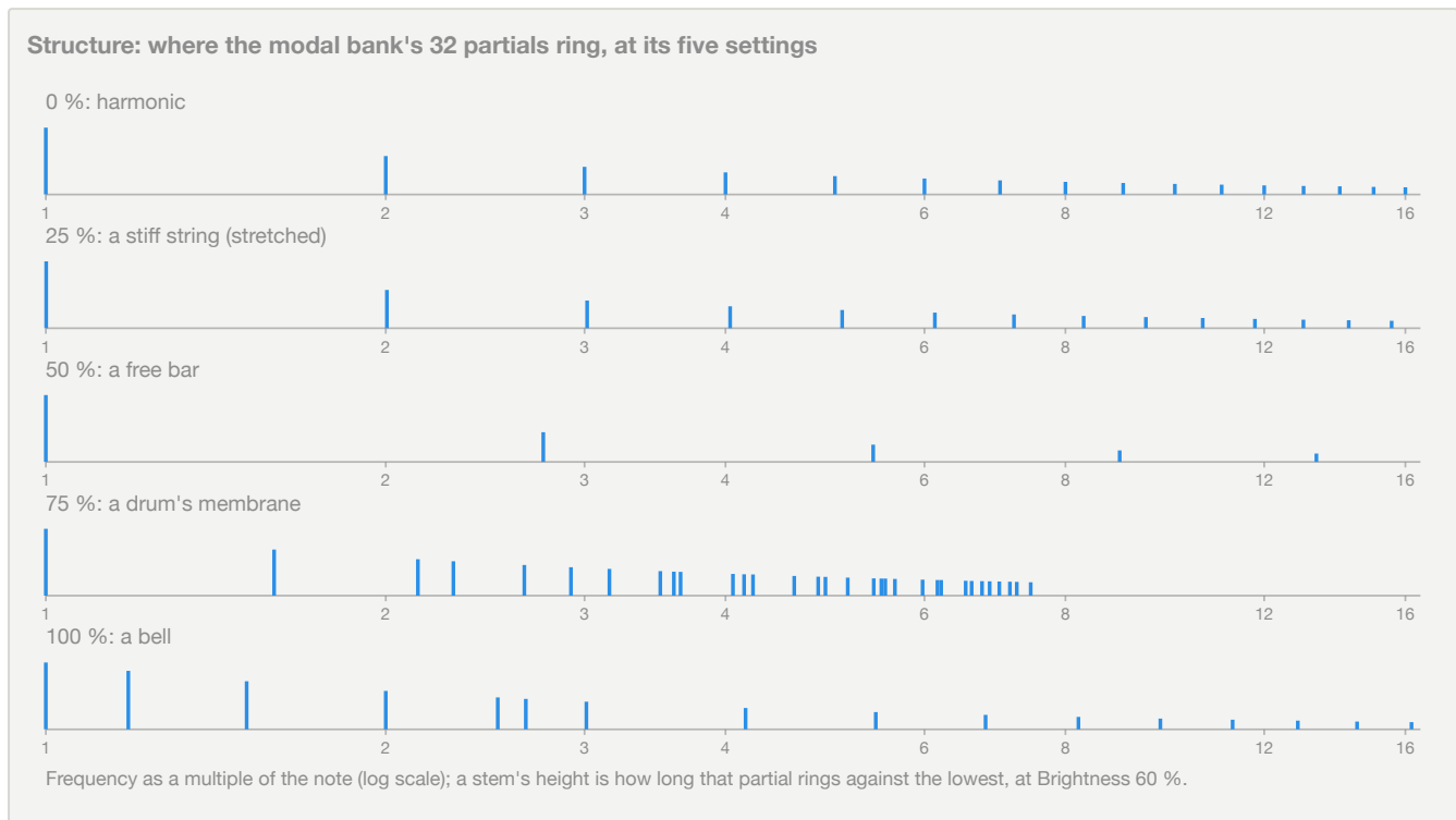
Structure: where the 32 partials ring, at its five settings
