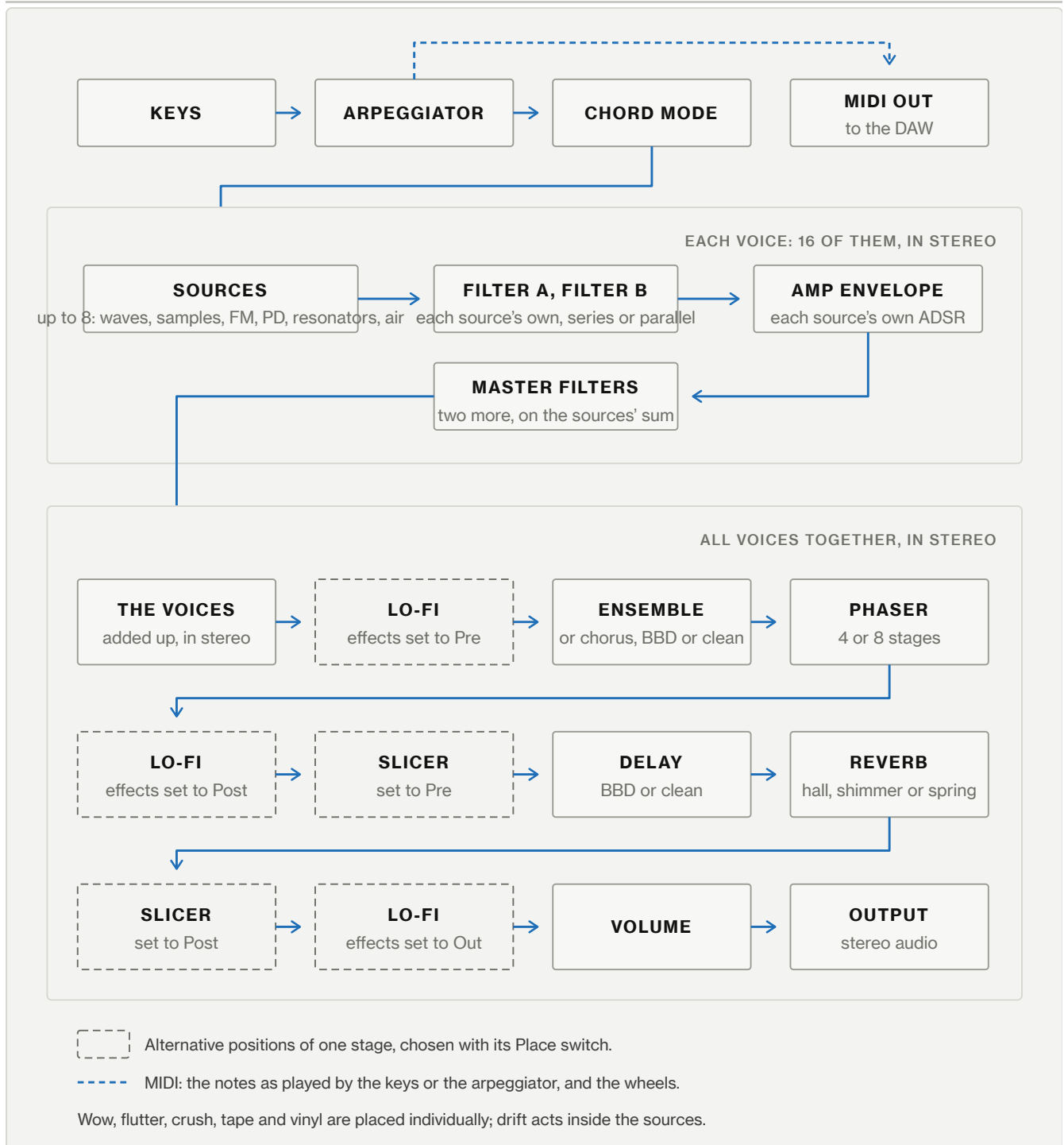
Signal path
